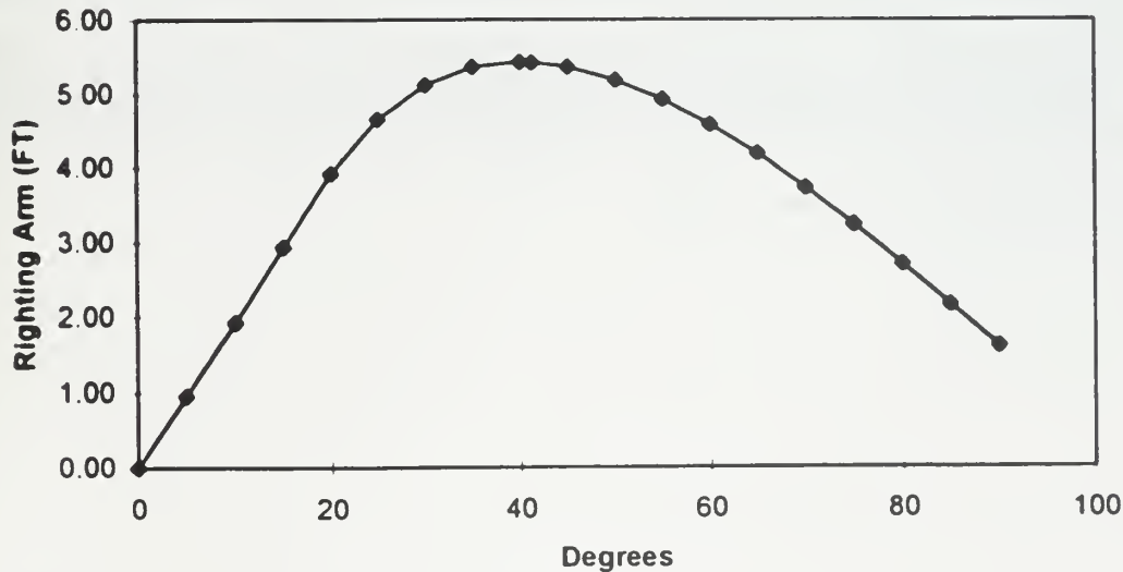
Figure 8. Wallsided Righting Arm Curve (Case II)
